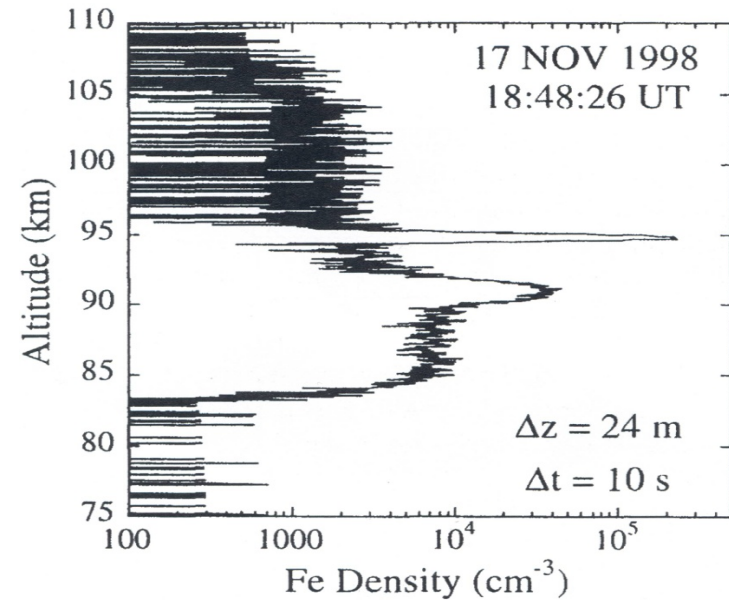
Profile on an Fe meteor trail measured by lidar [Chu et al. , GRL, 2000b]
