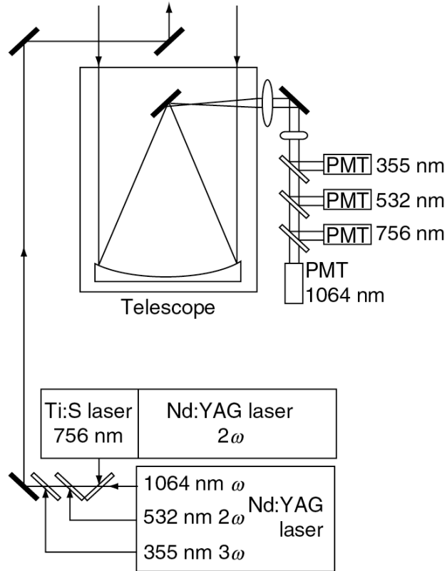
Block diagram of four-wavelength lidar.
