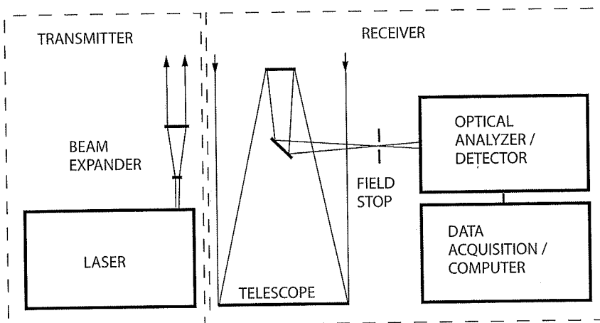
Fig. 1.1. Principle setup of a lidar system.
