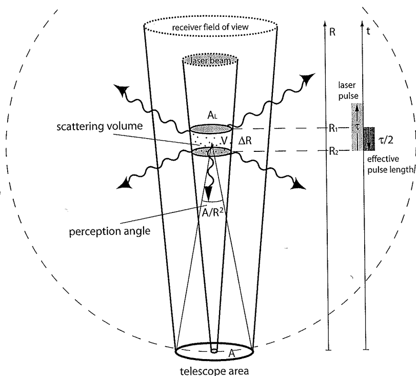
Fig. 1.2. Illustration of the lidar geometry.
